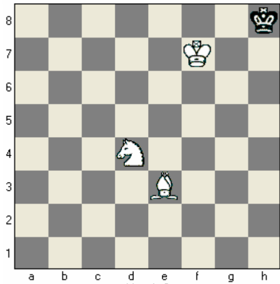
Mate in 3
