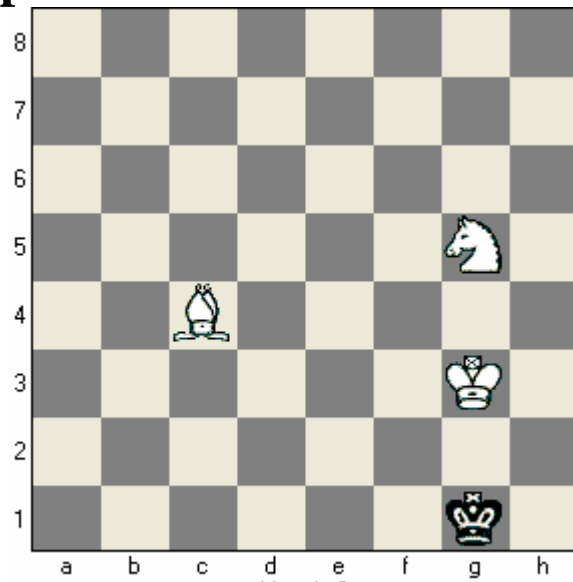
Mate in 2
